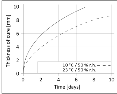
Diagram 1: Curing speed Sikaflex®-211 EN
