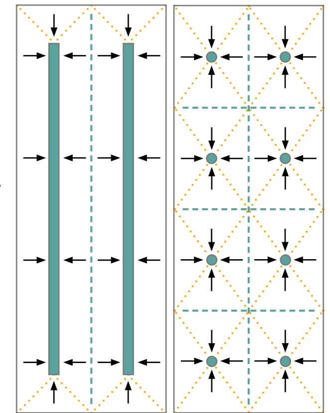
A floor designed with channels (figure on the left) is easier to build than a floor with isolated gulleys (figure on the right).
