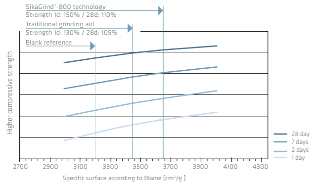
Strength enhancement with SikaGrind® due to increased fineness at constant production
