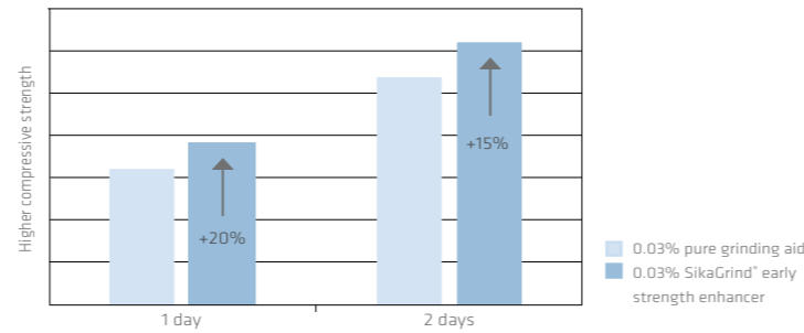
Strength enhancement with SikaGrind® due to optimized particle size distribution at constant production
